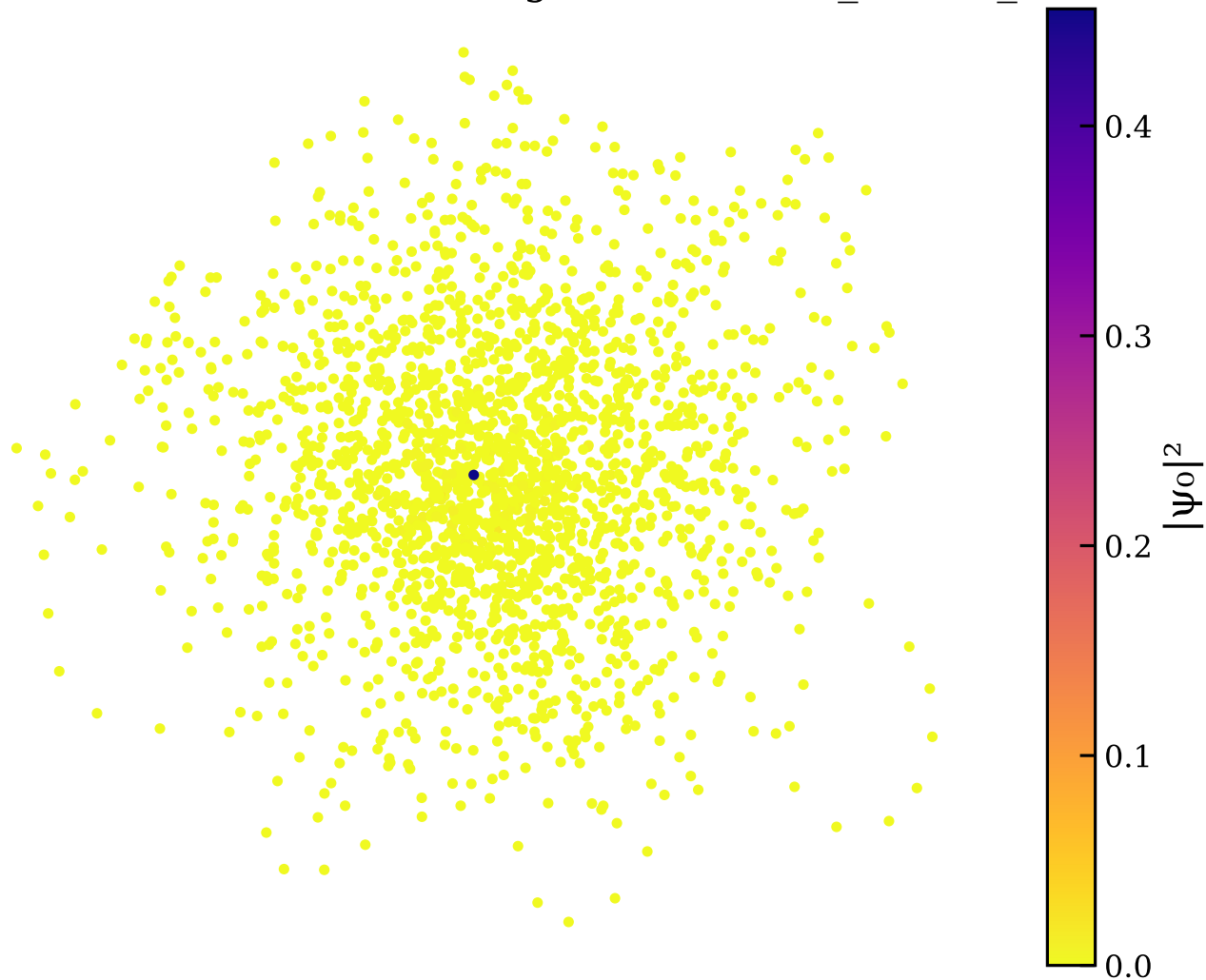
Ground state distribution: configuration model_N2000_G3
